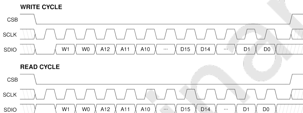
Figure 28: 3-wire SPI timing.
