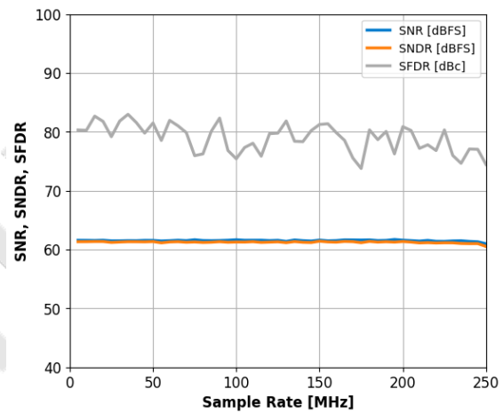
Figure 16: Single-Tone SNR, SNDR and SFDR vs. Sample Rate with f_{IN}=70.2\text{MHz} .
