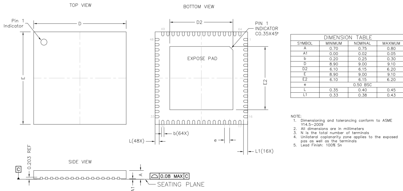
Figure 30: Package Dimensions.
