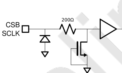
Figure 21: Equivalent CSB or SCLK Input Circuit.
