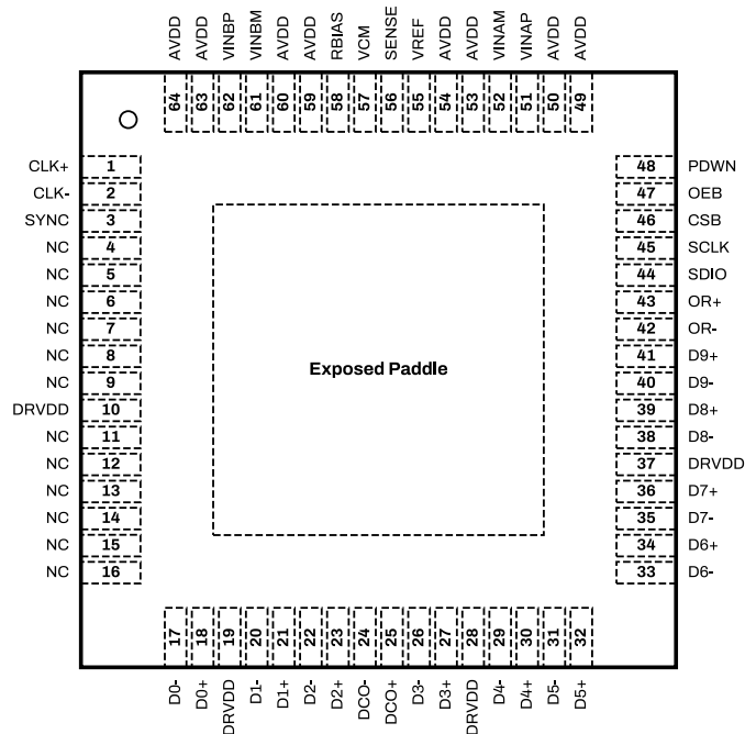
Figure 5: SD0802 Package Top View for Channel Multiplexed LVDS Configuration.
