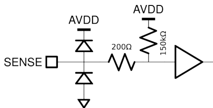
Figure 27: Equivalent SENSE Input Circuit.
