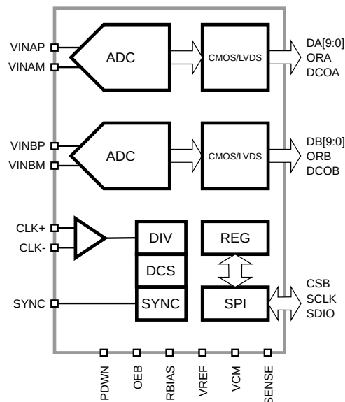
Figure 1: SD0802 Functional Block Diagram.
