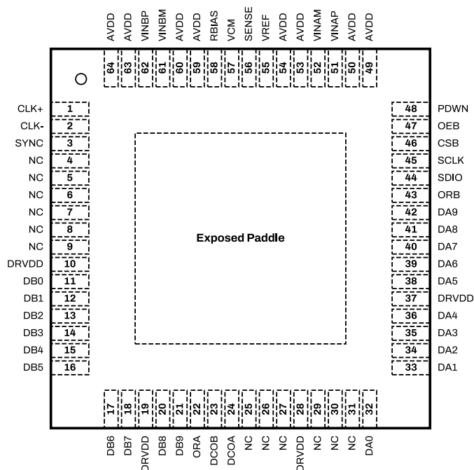
Figure 6: SD0802 Package Top View for Parallel CMOS Configuration.
