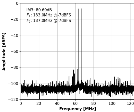
Figure 11: Two-Tone FFT with f_{IN1}=183.0\text{MHz} , f_{IN2}=187.0\text{MHz} .
