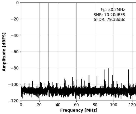
Figure 7: Single-Tone FFT with f_{IN}=30.2\text{MHz} .
