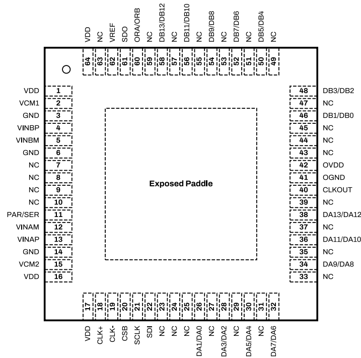
Figure 6: SD2140ET Package Top View for Channel Multiplexed CMOS Configuration.
