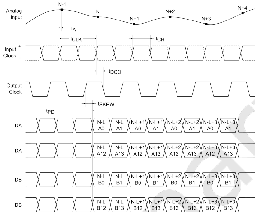
Figure 3: Channel Multiplexed CMOS Output Mode Timing.
