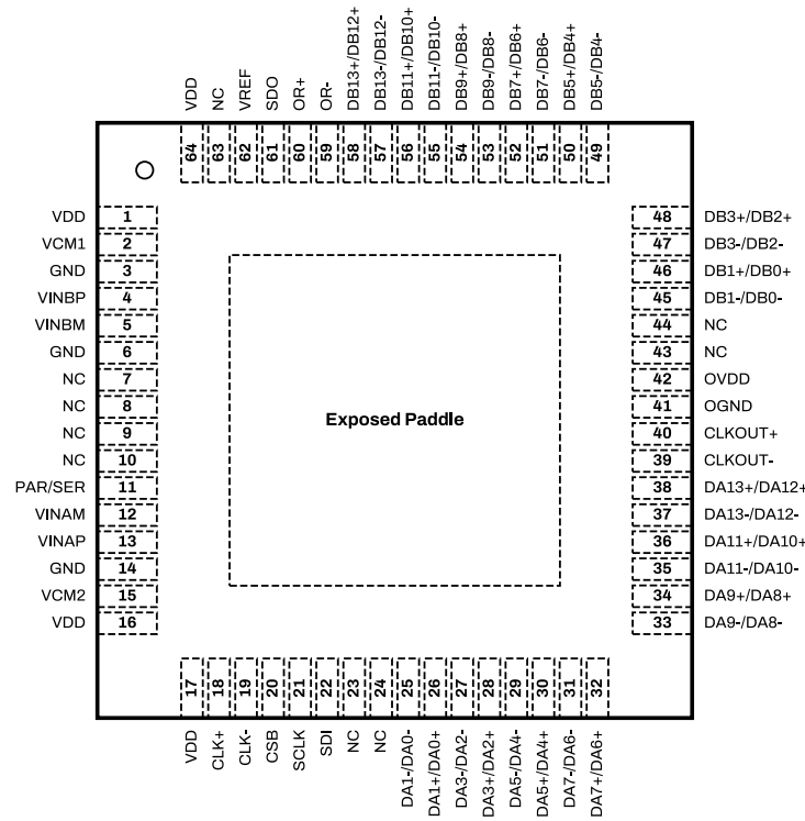
Figure 7: SD2140ET Package Top View for Channel Multiplexed LVDS Configuration.
