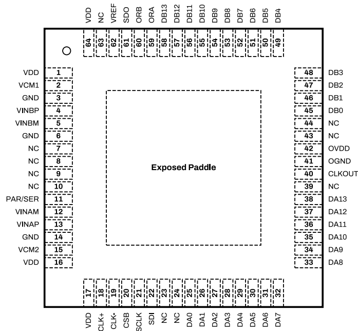
Figure 5: SD2140ET Package Top View for Parallel CMOS Configuration.
