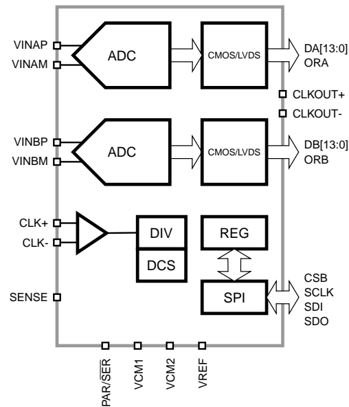
Figure 1: SD2140ET Functional Block Diagram.
