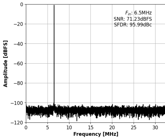
Figure 8: Single-Tone FFT with f_{IN}=6.55\text{MHz} .
