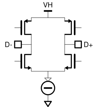
Figure 25: Equivalent LVDS output Circuit.
