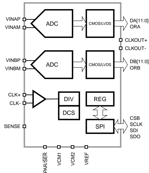
Figure 1: SD2143ET Functional Block Diagram.
