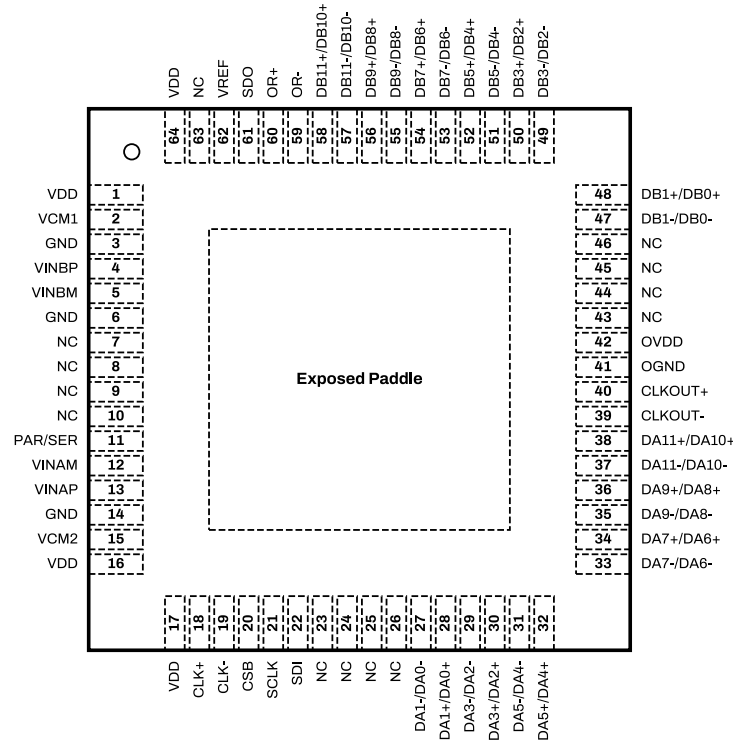
Figure 7: SD2143ET Package Top View for Channel Multiplexed LVDS Configuration.
