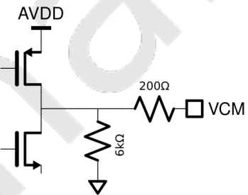
Figure 23: Equivalent VCM Circuit.
