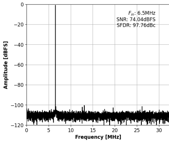
Figure 6: Single-Tone FFT with f_{IN}=6.55\text{MHz} .
