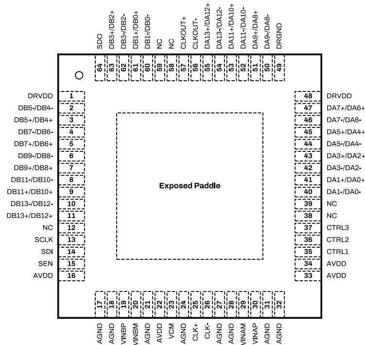
Figure 5: SD4242ET Package Top View for Channel Multiplexed LVDS Configuration.
