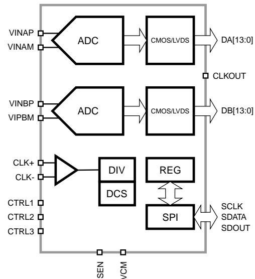
Figure 1: SD4242ET Functional Block Diagram.
