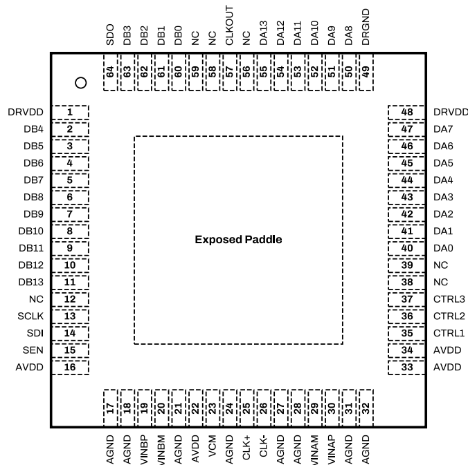
Figure 4: SD4242ET Package Top View for Parallel CMOS Configuration.
