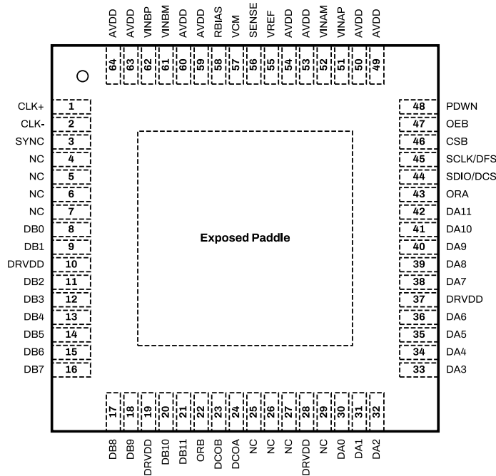
Figure 5: SD9231ET Package Top View for Parallel CMOS Configuration.
