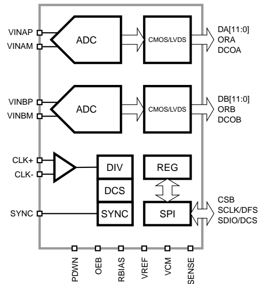
Figure 1: SD9231ET Functional Block Diagram.
