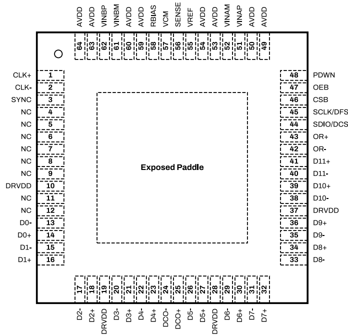
Figure 6: SD9231ET Package Top View for Parallel LVDS Configuration.
