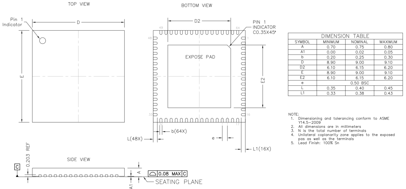
Figure 32: Package Dimensions.
