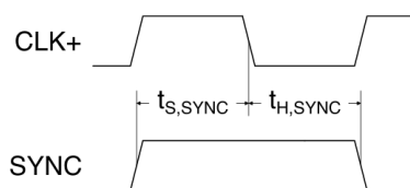
Figure 2: SYNC Input Timing.
