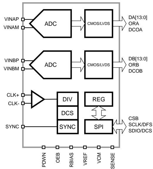
Figure 1: SD9258ET Functional Block Diagram.
