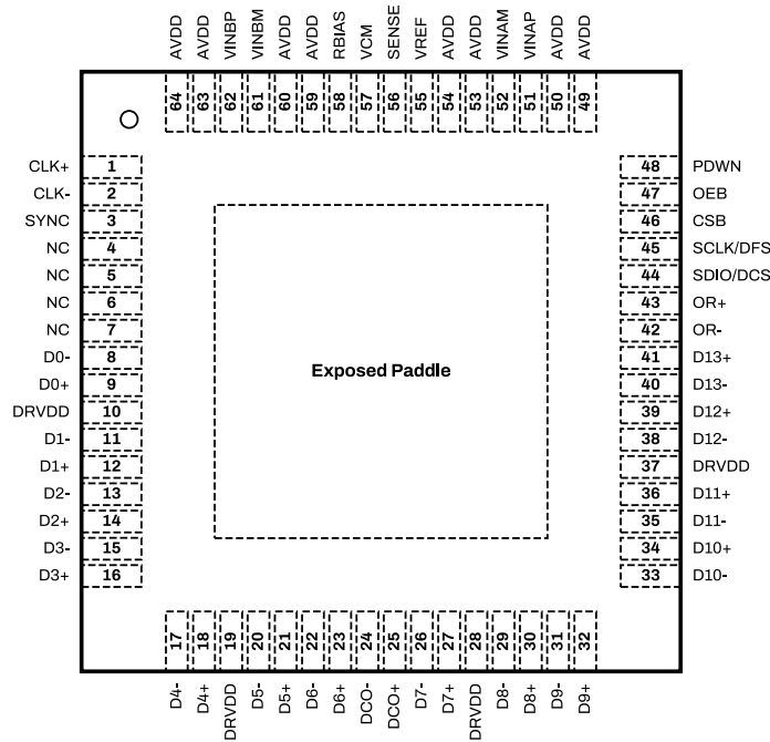
Figure 6: SD9258ET Package Top View for Parallel LVDS Configuration.
