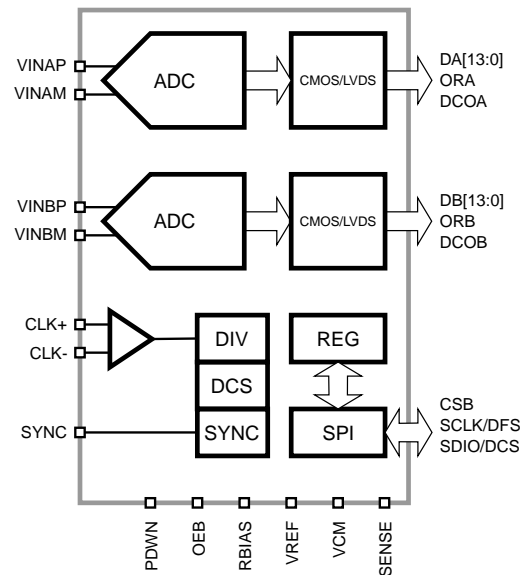
Figure 1: SD9258ET Functional Block Diagram.
