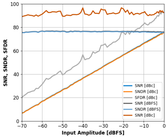
Figure 15: Single-Tone SNR, SNDR and SFDR vs. Input Amplitude with f_{IN}=30.2\text{MHz} .
