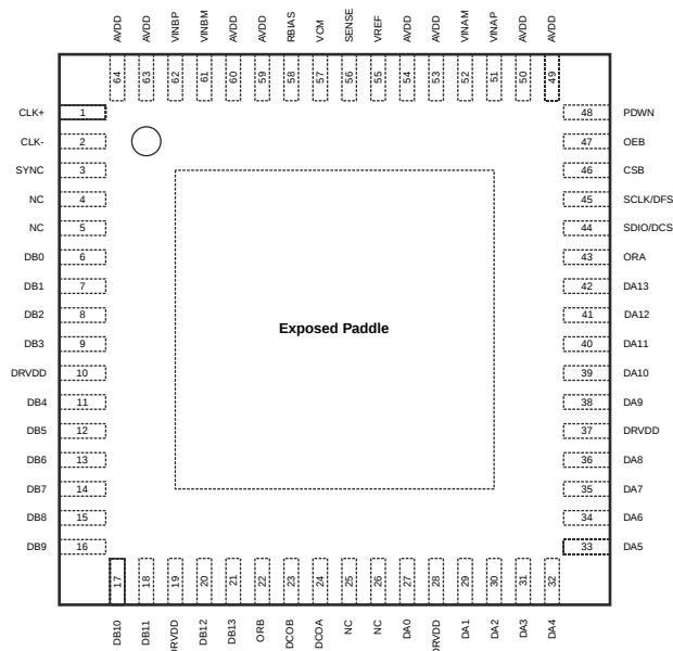
Figure 5: SD9258 Package Top View for Parallel CMOS Configuration.
