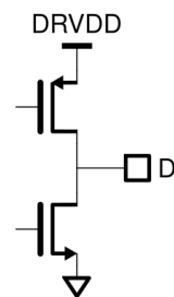
Figure 25: Equivalent Digital Output Circuit.
