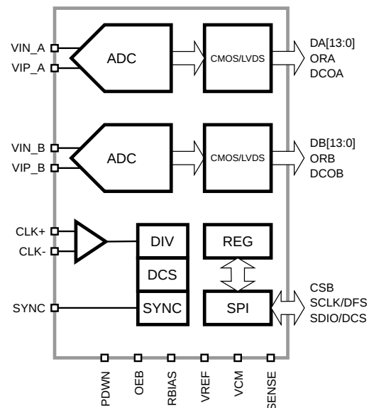
Figure 1: SD9258 Functional Block Diagram.
