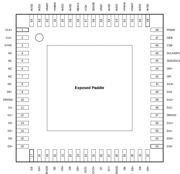
Figure 6: SD9258 Package Top View for Parallel LVDS Configuration.
