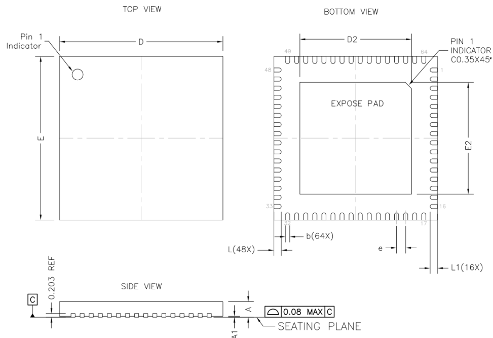
Figure 30: Package Dimensions.
