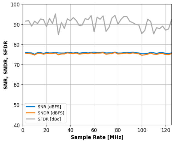
Figure 17: Single-Tone SNR, SNDR and SFDR vs. Sample Rate with f_{IN}=30.2\text{MHz} .
