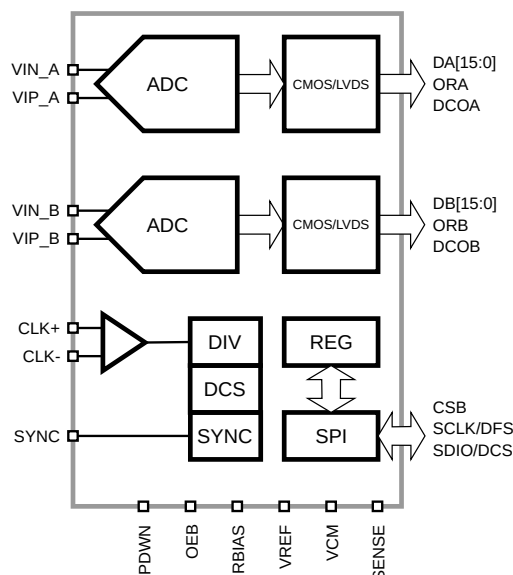
Figure 1: SD9268 Functional Block Diagram.
