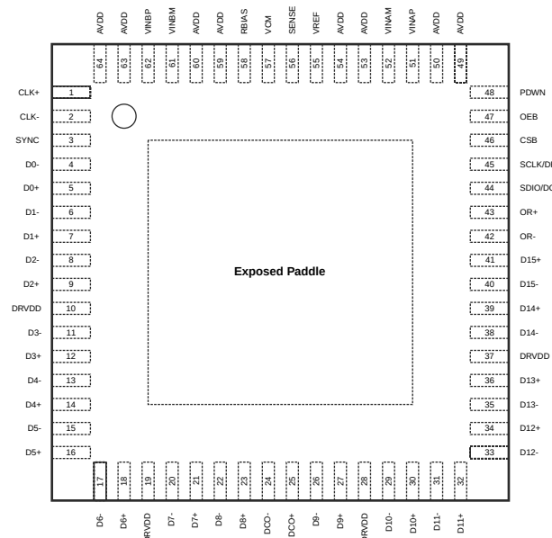
Figure 6: SD9268 Package Top View for Parallel LVDS Configuration.
