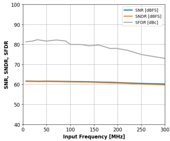
Figure 12: Single-Tone SNR, SNDR and SFDR vs. Input Frequency with f_S=40\text{MHz} .
