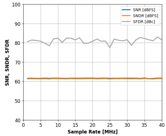
Figure 13: Single-Tone SNR, SNDR and SFDR vs. Sample Rate with f_{IN}=30.2\text{MHz} .
