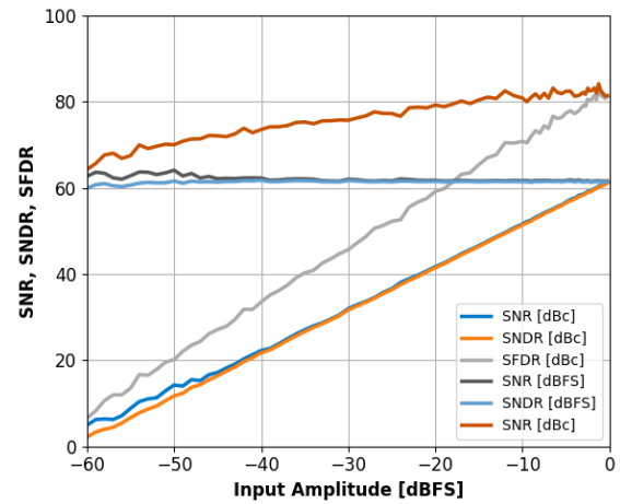
Figure 11: Single-Tone SNR, SNDR and SFDR vs. Input Amplitude with f_{IN}=30.2\text{MHz} .
