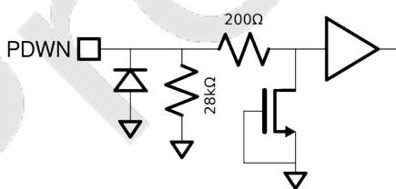
Figure 27: Equivalent PDWN Input Circuit.
