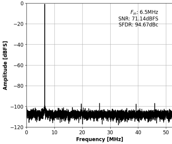
Figure 9: Single-Tone FFT with f_{IN}=6.55\text{MHz} .
