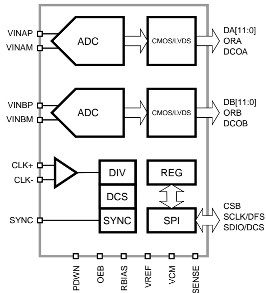
Figure 1: SD9628ET Functional Block Diagram.
