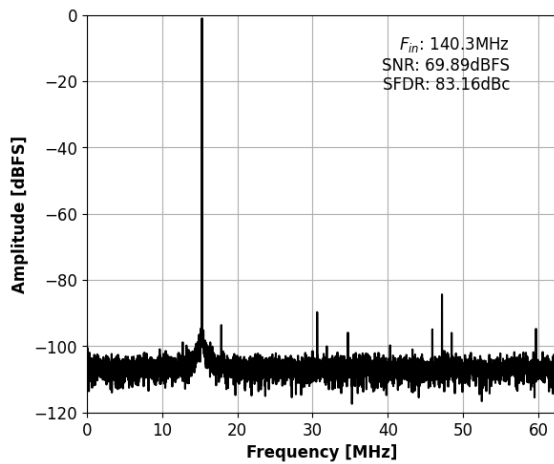
Figure 11: Single-Tone FFT with f_{IN}=140\text{MHz} .
