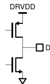
Figure 28: Equivalent Digital Output Circuit.
