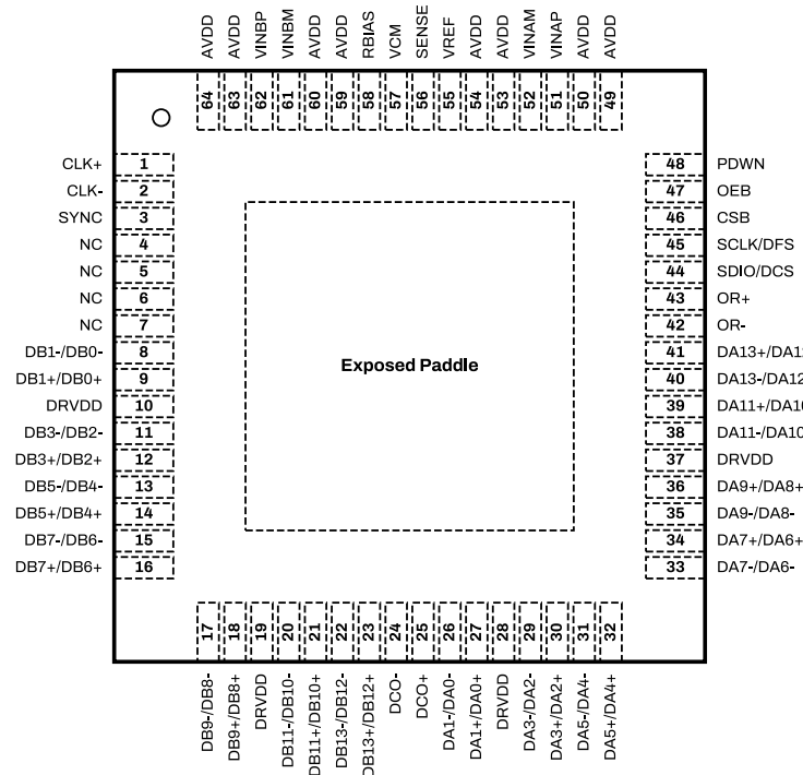
Figure 8: SD9648ET Package Top View for Channel Multiplexed LVDS Configuration.
