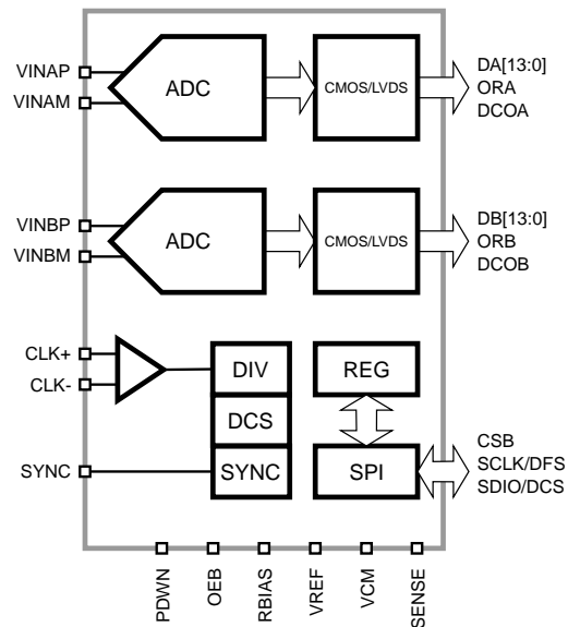
Figure 1: SD9648ET Functional Block Diagram.
