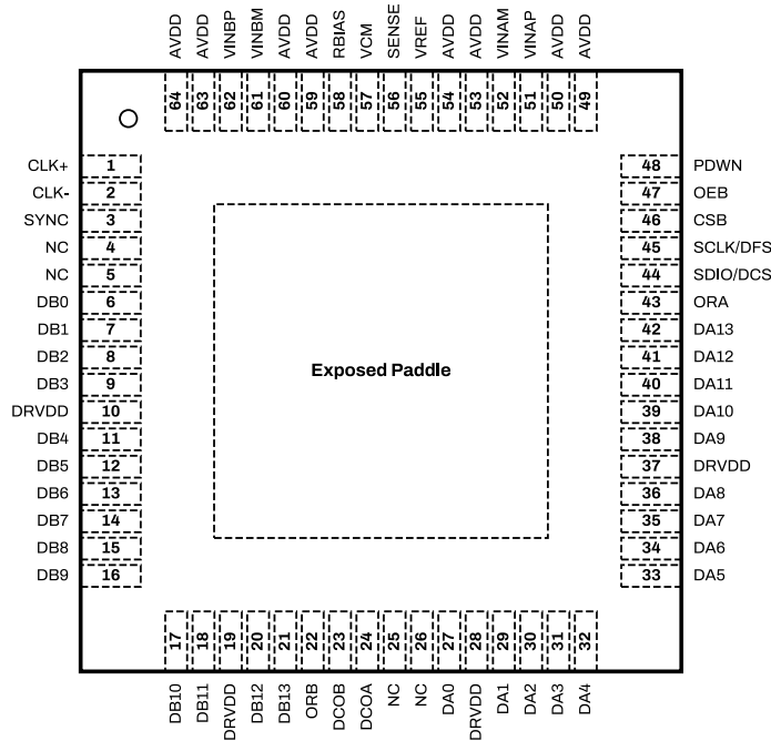
Figure 6: SD9648ET Package Top View for Parallel CMOS Configuration.
