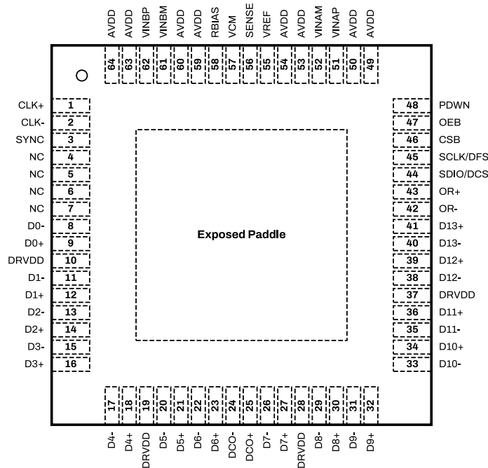
Figure 7: SD9648ET Package Top View for Interleaved Parallel LVDS Configuration.
