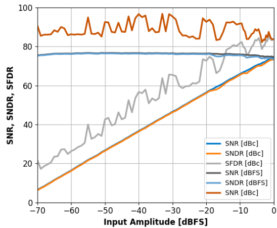
Figure 17: Single-Tone SNR, SNDR and SFDR vs. Input Amplitude with f_{IN}=70.2\text{MHz} .
