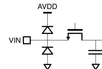
Figure 21: Equivalent Analog Input Circuit.
